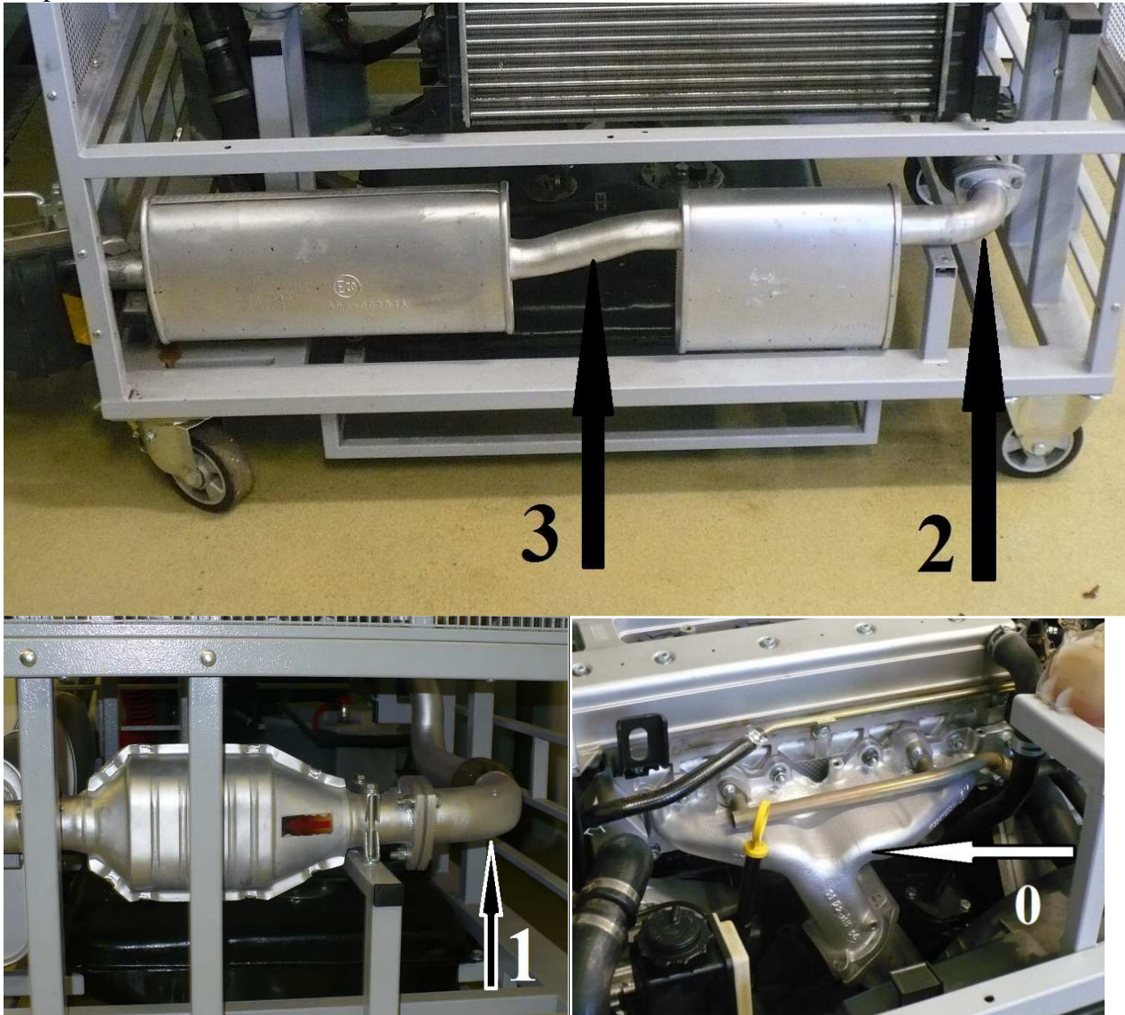
Fig. 2. Photos presenting the measuring points.
