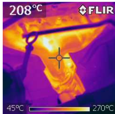
Fig. 3. Photo of the 0 measurement point. for 2000 rpm
