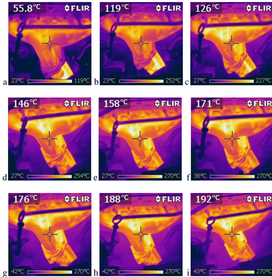
Fig. 11. Photos of the heating point "0" registered at two-minute time intervals.
