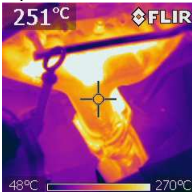
Fig. 7. Photo of the 0 measurement point. for 3000 rpm
